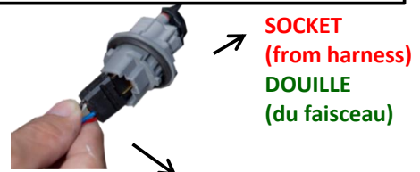
SOCKET (from harness) DOUILLE (du faisceau) PLUG (from new taillight) PRISE (du nouveau feu)
